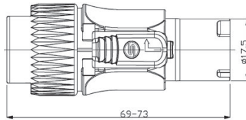
Neutrik NAC3FX-Compatible Locking Female Cable Connector
