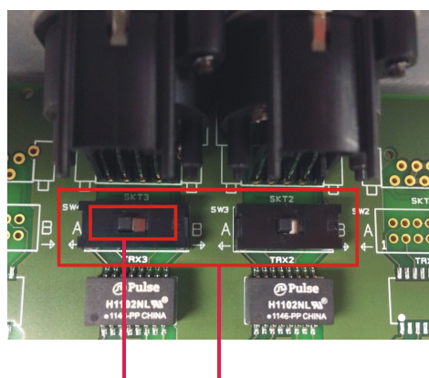
Position A for console use MADi DMI C internal switches
